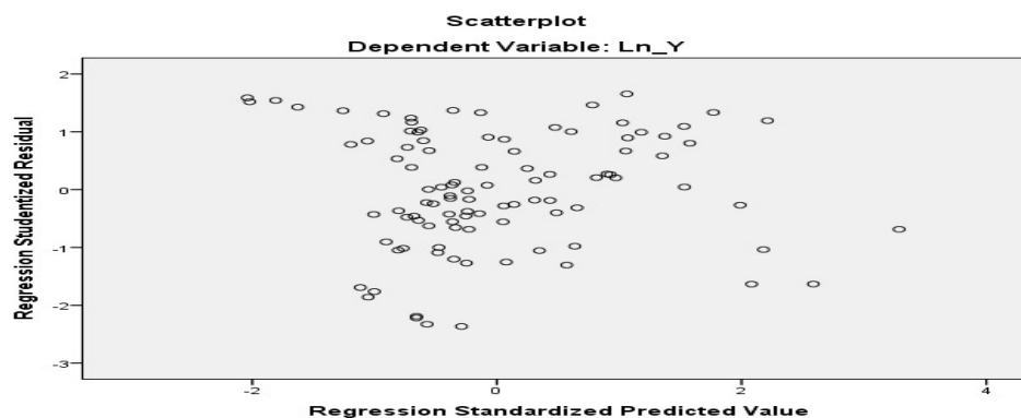
Figure 1. Scatterplot test
